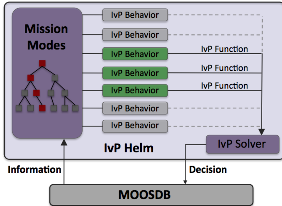
FIGURE 2.4 – The hierarchical mission structure using the IvP helm application. In the .bhv it is possible to declare mission modes that uses a set of behaviors. The IvP solver resolves possible conflicts (MOOS-IVP, 2016).
