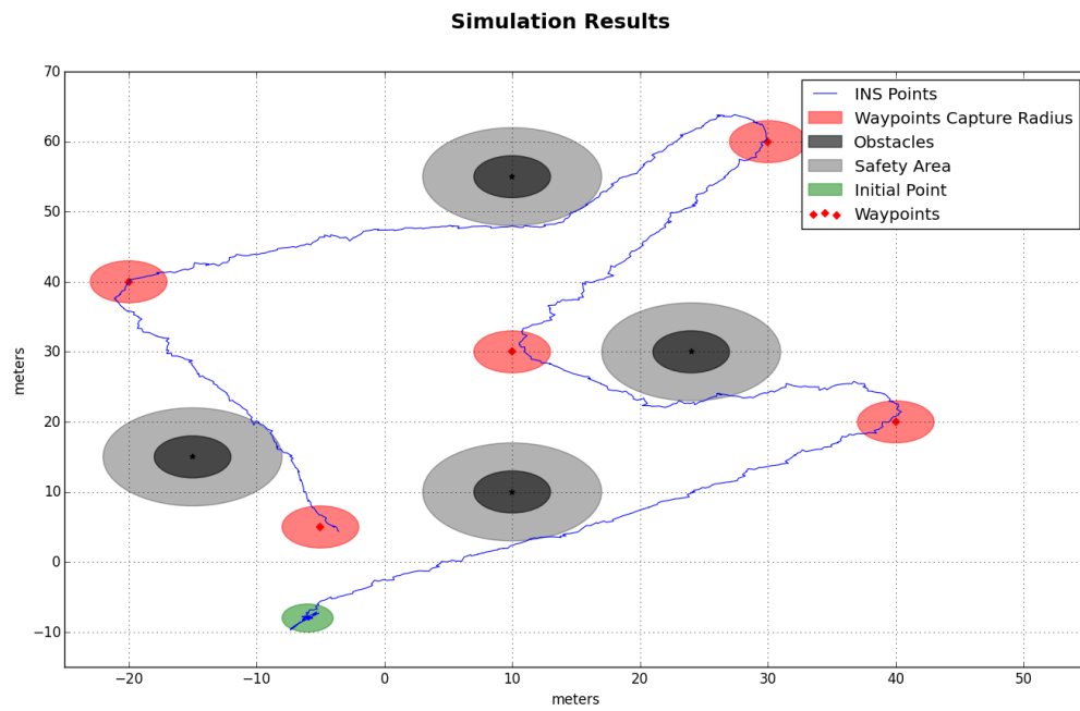
FIGURE 5.2 – Simulation results obtained using the boat model with the uBoatSimulator application.
