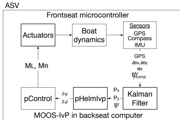
FIGURE 3.13 – This block diagram shows how the Kalman Filter is used for the sensor fusion. It receives GPS, IMU and compass data (through the application iSerial), it processes those data and outputs the estimated position and heading to the pHelmIvp.
