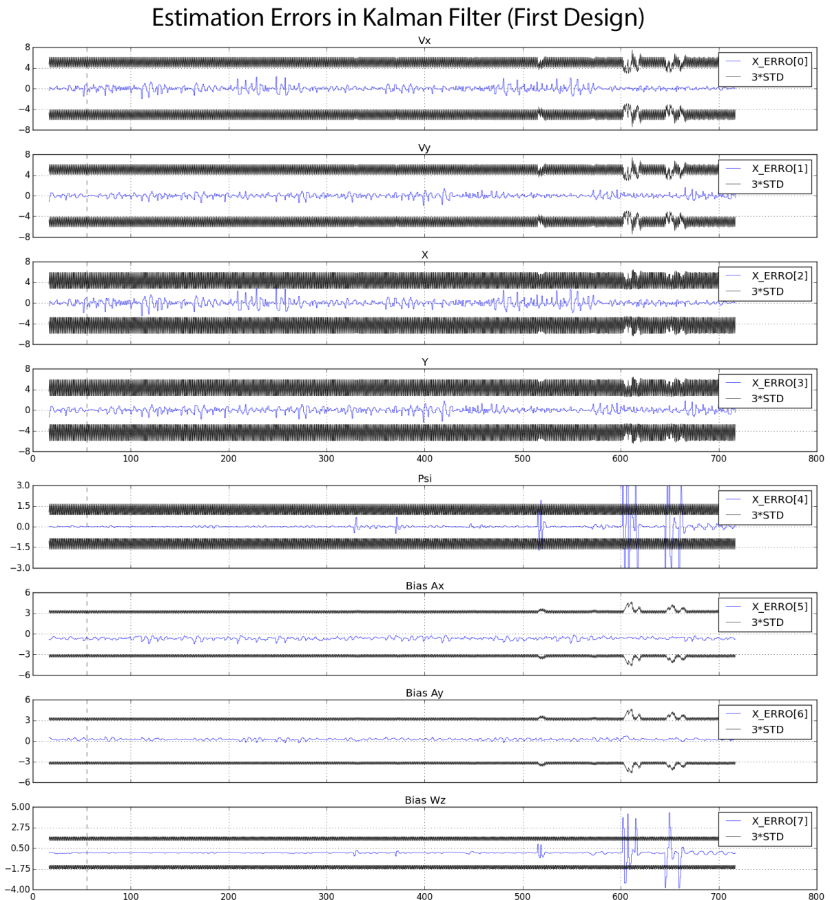
FIGURE 5.5 – The Kalman Filter errors in the first design field experiment. The blue line represents the estimated error of the Kalman Filter. The black line represents the standard deviation ( \pm 3\sigma ). This figure presents the same information that can be seen in real-time using the uKalmanVisual application.
