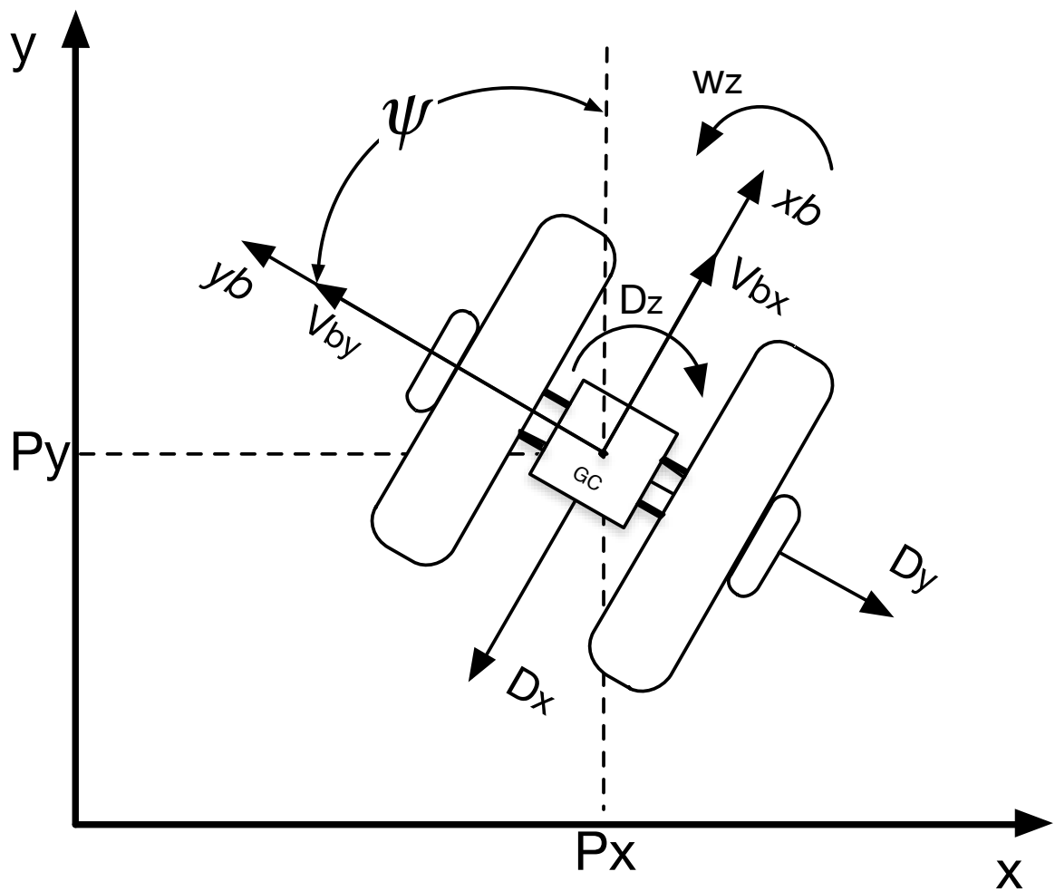
FIGURE 3.2 – A diagram representing the model of the ASV. This diagram shows the ASV frame axis, the local frame axis, the velocities and drag forces.
