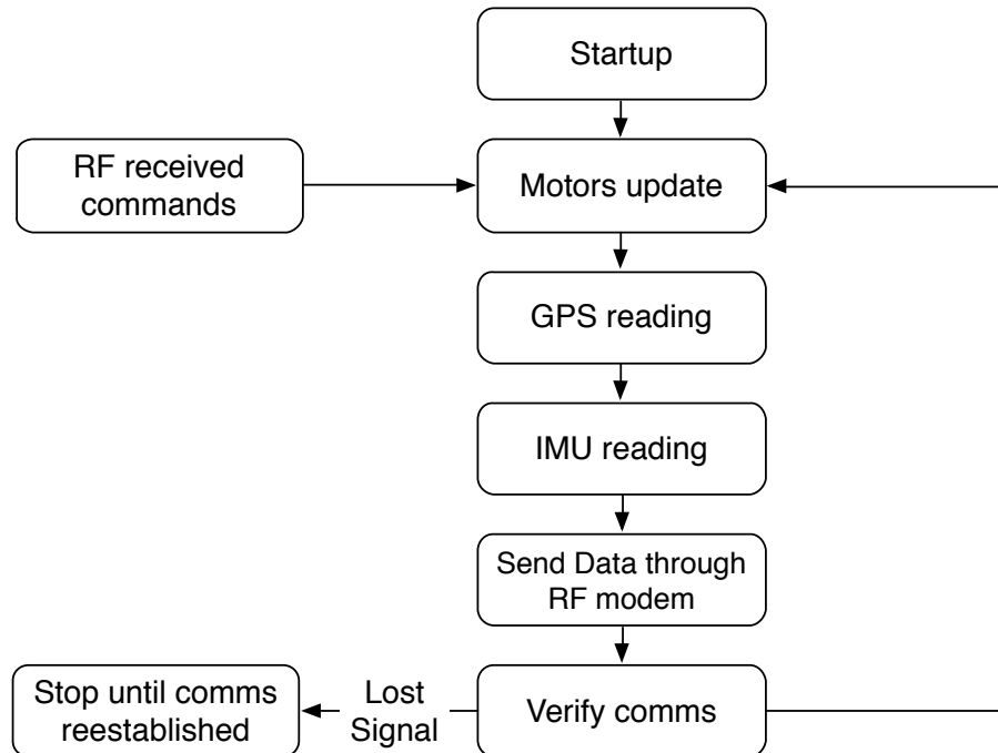
FIGURE 3.6 – Arduino embedded software. The software is composed of a single main loop that controls the motors, reads sensors and sends telemetry data.
