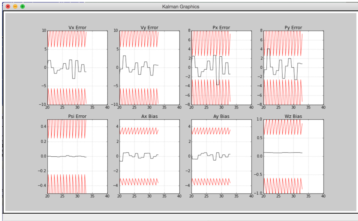
FIGURE 4.2 – A screen capture of the uKalmanVisual application. The red lines represent the \pm 3\sigma plots and the black lines represent the error of each variable. If the error stays most of the time in the \pm 3\sigma region for every value it can be said that filter converges.
