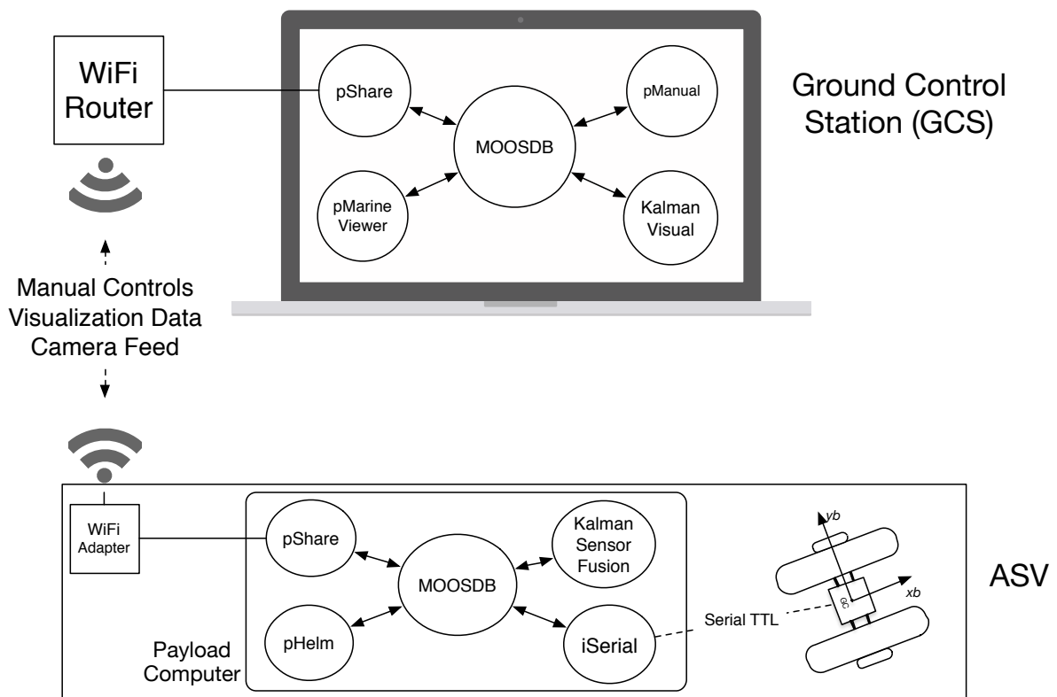
FIGURE 3.9 – Block diagram of the AVS system: the ASV and the GCS. Both the GCS and the ASV use the MOOS-IvP software. Communication between the ASV and the GCS happens through a WiFi link.
