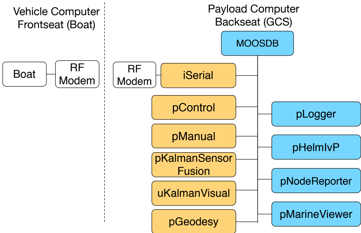
FIGURE 3.7 – MOOS-IvP Apps. In yellow, the custom MOOS Apps developed for the ASV. In blue, the MOOS Apps available in the MOOS-IvP repository.
