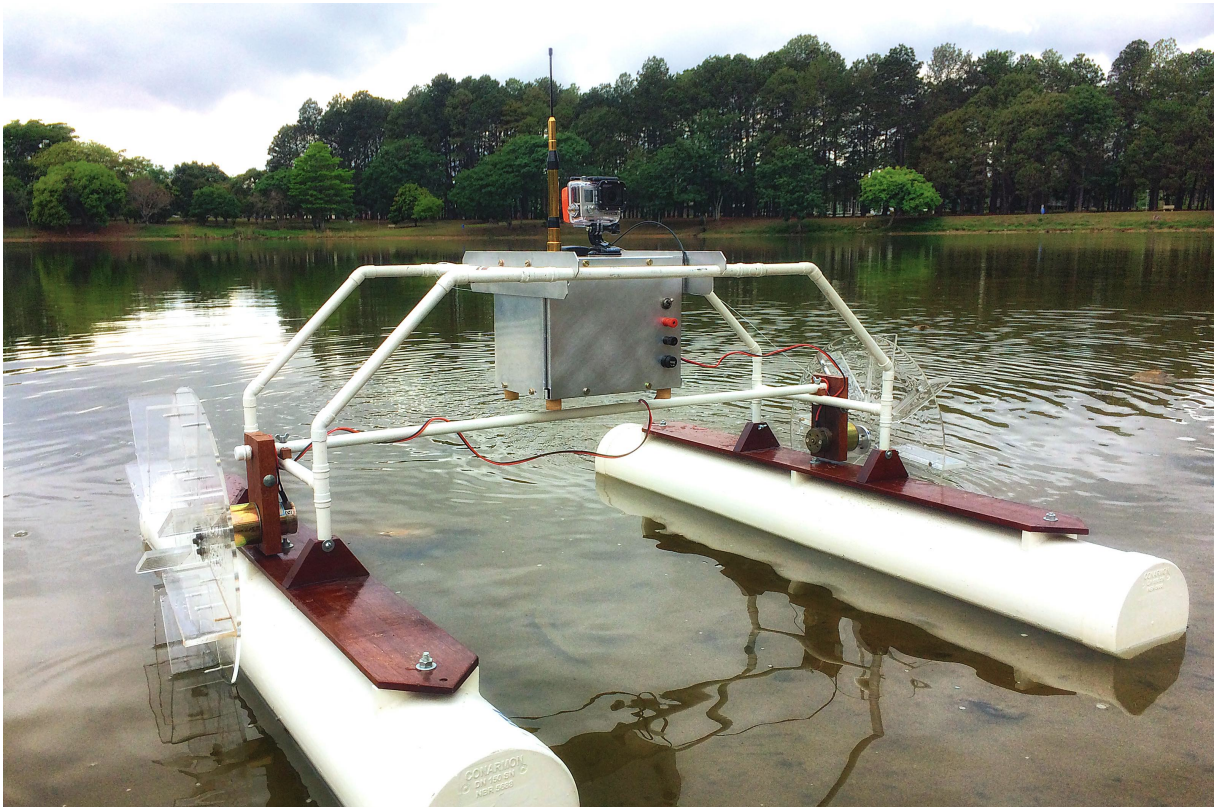
FIGURE 3.1 – A photograph of the catamaran boat used in this dissertation. The embedded hardware is contained inside the metal box.
