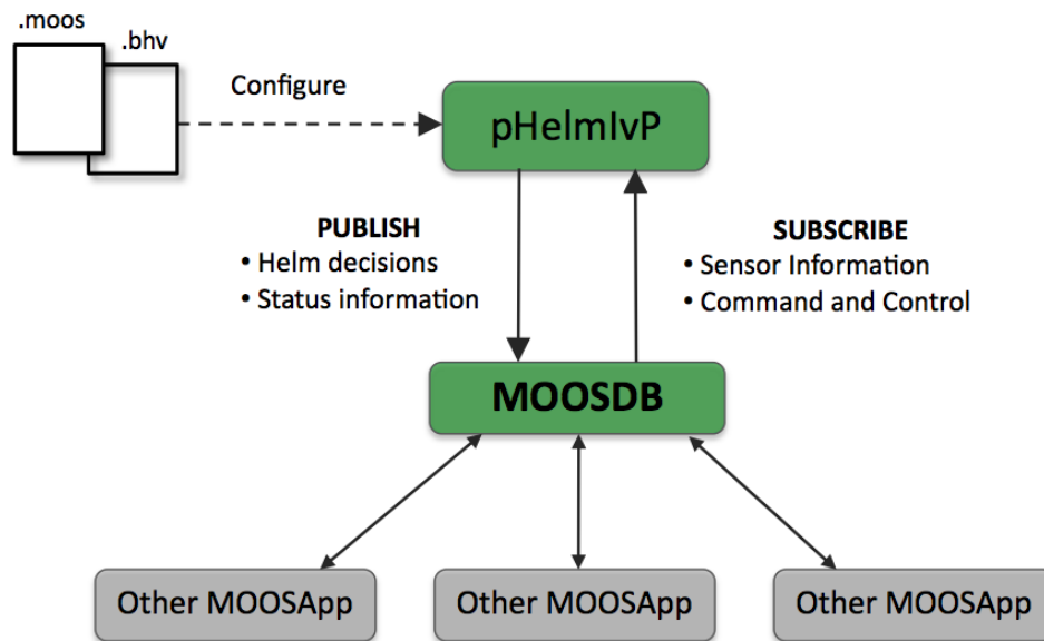
FIGURE 2.3 – The IvP helm as a MOOS application (MOOS-IVP, 2016).
