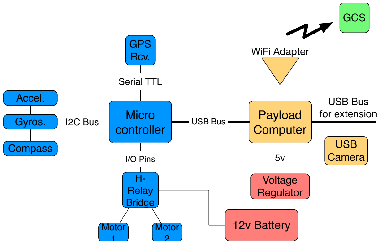
FIGURE 3.10 – Block diagram of the AVS hardware. In blue is represented the embedded hardware, in yellow the payload computer, in red the power source. In green is represented the GCS.
