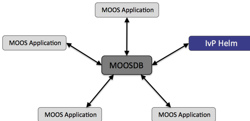
FIGURE 2.2 – Star topology for the MOOS Software (MOOS-IVP, 2016).
