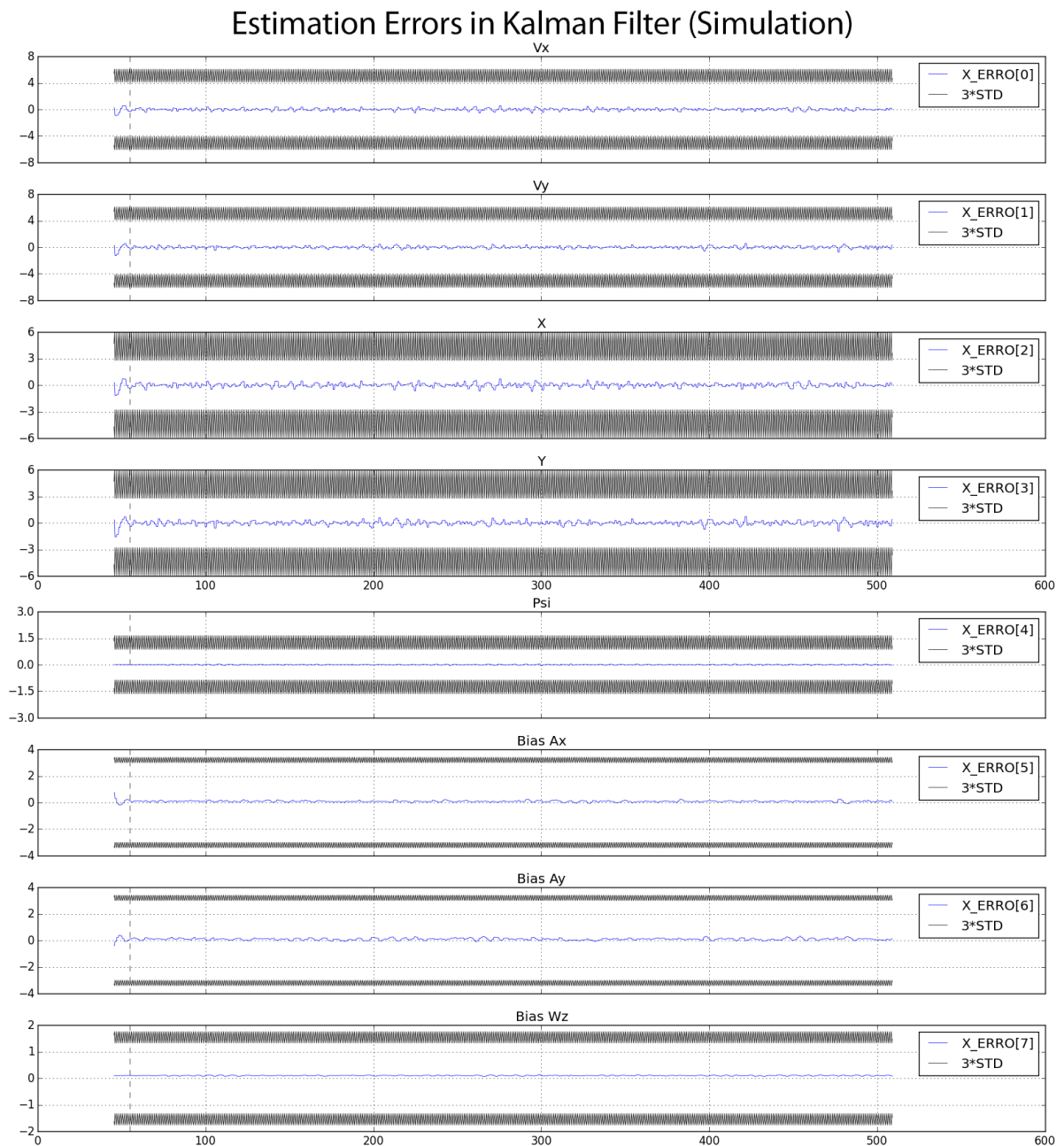
FIGURE 5.3 – The Kalman Filter errors in the simulation environment. The blue line represents the estimated error of the Kalman Filter. The black line represents the standard deviation ( \pm 3\sigma ). This figure presents the same information that can be seen in real-time using the uKalmanVisual application.
