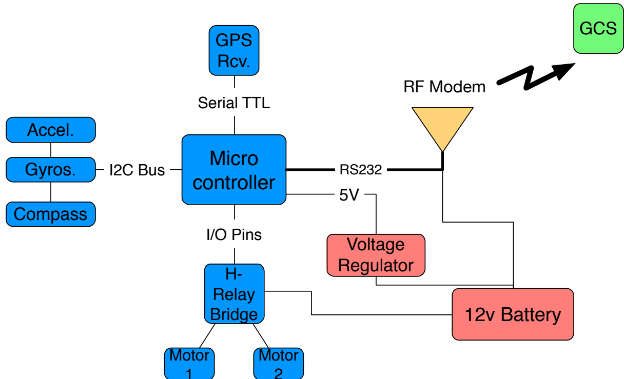
FIGURE 3.4 – Diagram of the ASV embedded hardware in the first design. In blue is represented the embedded hardware. In red the power source. In green the communication to the GCS.
