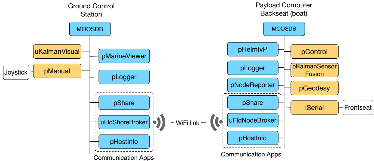
FIGURE 3.12 – MOOS-IvP Apps. In the left there is a diagram of the MOOS apps used in the GCS, in the right the diagram for the MOOS apps used in the payload computer. The yellow blocks correspond to the custom MOOS Apps developed for the ASV. The blue blocks correspond to the MOOS Apps available in the MOOS-IvP repository.
