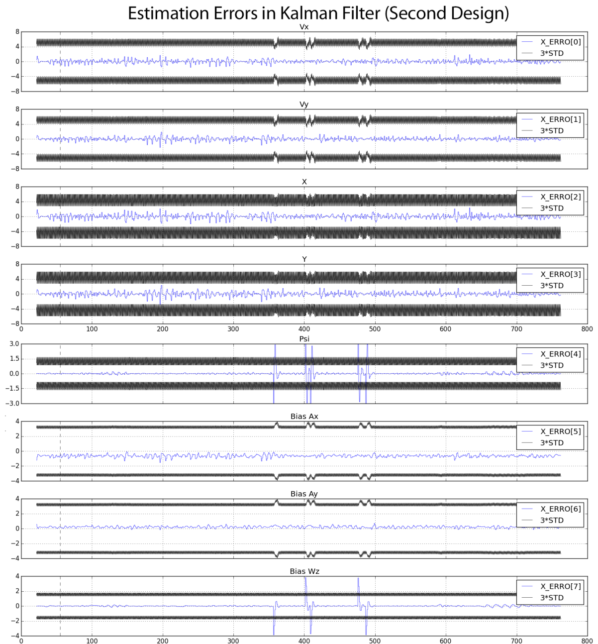
FIGURE 5.7 – The Kalman Filter errors in the second design field experiment. The blue line represents the estimated error of the Kalman Filter. The black line represents the standard deviation ( \pm 3\sigma ). This figure presents the same information that can be seen in real-time using the uKalmanVisual application.
