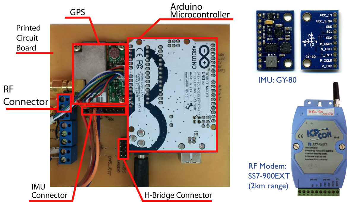
FIGURE 3.5 – Embedded hardware.
