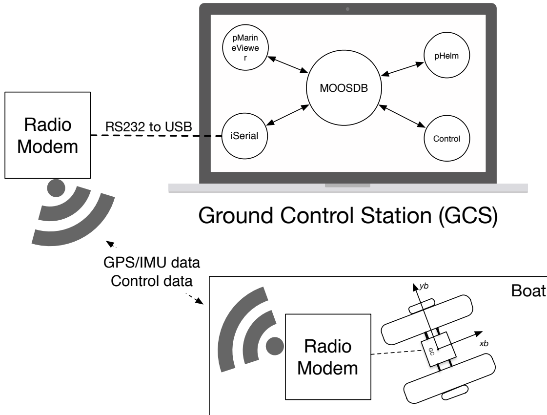
FIGURE 3.3 – The AVS system: the boat sends telemetry data to the GCS, the GCS process these data using the software MOOS-IvP and replies with navigation commands.
