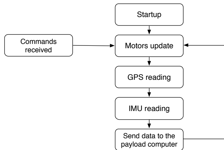
FIGURE 3.11 – Arduino embedded software. The software is composed of a single main loop that controls the motors, reads the sensors and communicates with the payload computer.
