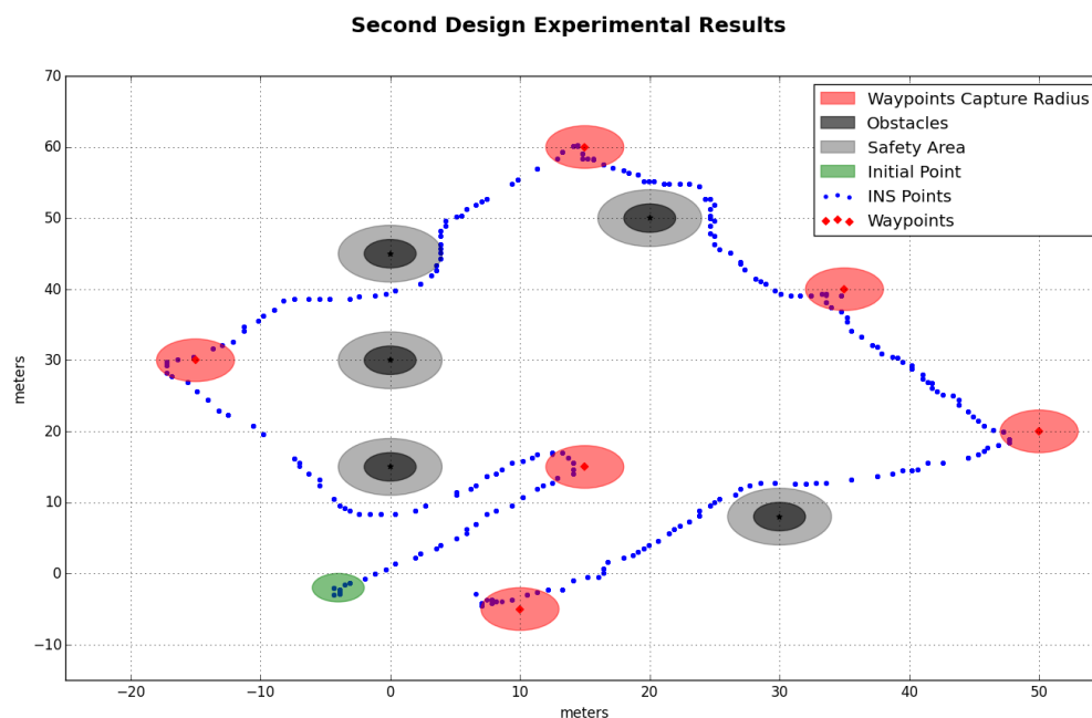
FIGURE 5.6 – Experimental results using the ASV in a lake. The vehicle is set to perform a mission consisting of several waypoints with virtual obstacles.
