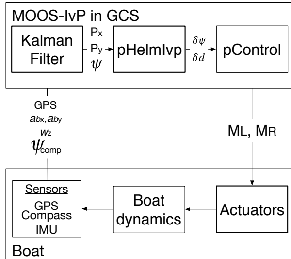
FIGURE 3.8 – This block diagram shows how the Kalman Filter is used for the sensor fusion. The GCS receives GPS, IMU and compass data (through the application iSerial), it processes those data and outputs the estimated position and heading to the pHelmIvp.
